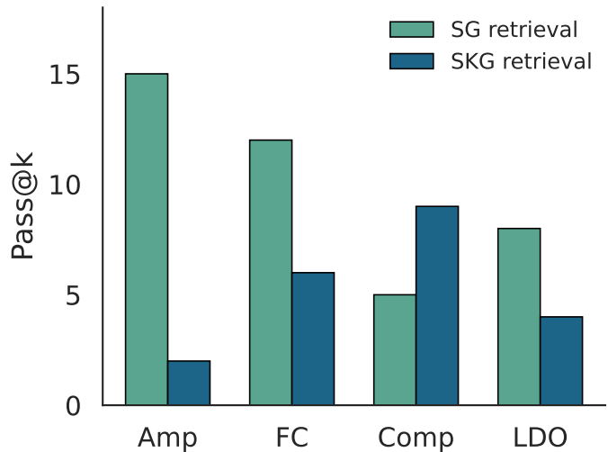
Top-k Retrieval
