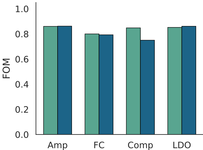
Bottom-k Retrieval
