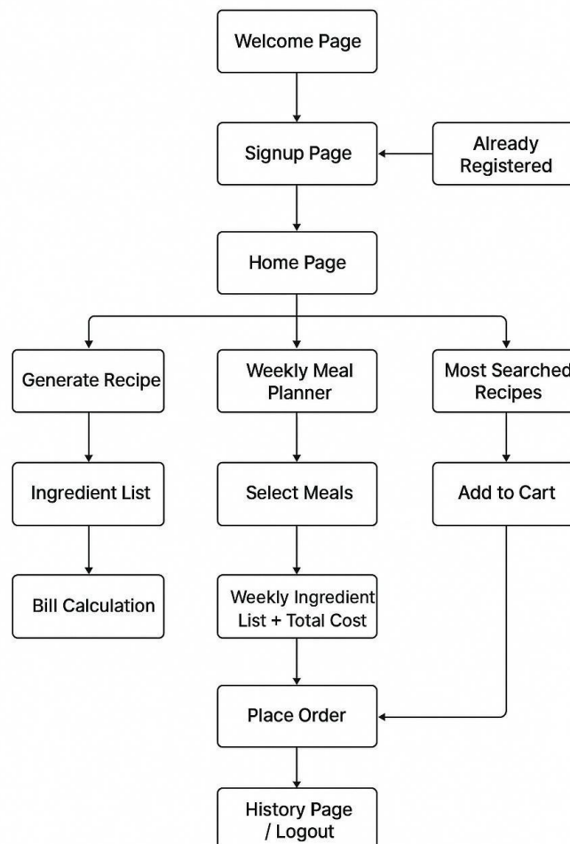
Flowchart of the Smart Grocery List Generator
