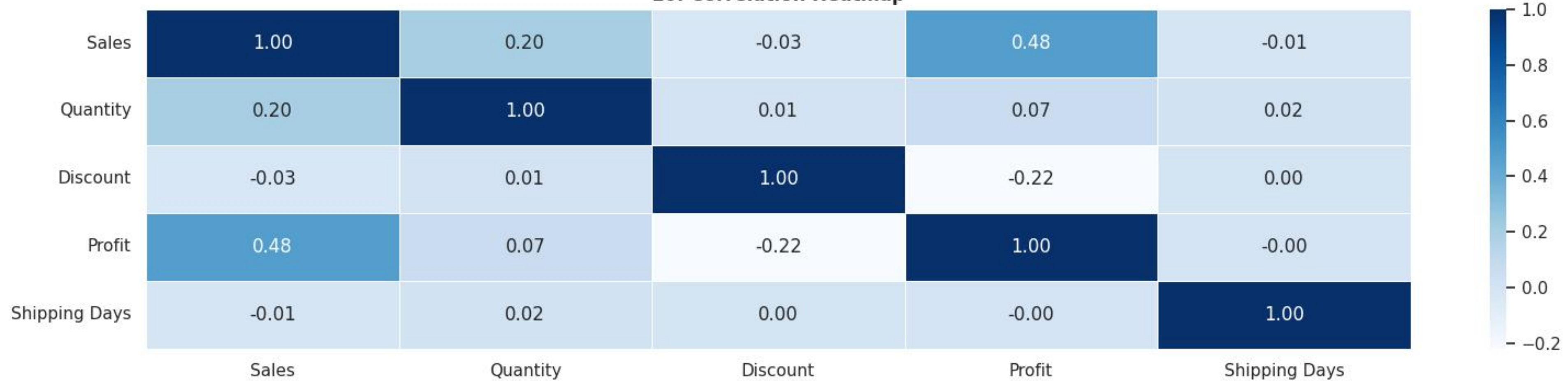
10. Correlation Heatmap
