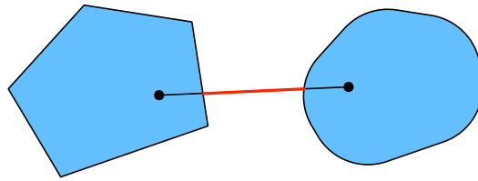
Fig. 12.2.3 The union of two convex sets need not be convex.
