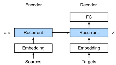
Fig. 10.7.2 Layers in an RNN encoder–decoder model.
