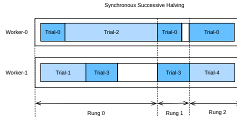
Fig. 19.5.1 Synchronous successive halving with two workers.
