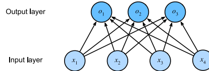
Fig. 4.1.1 Softmax regression is a single-layer neural network.
