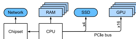
Fig. 13.4.2 Connectivity of components of a computer.
