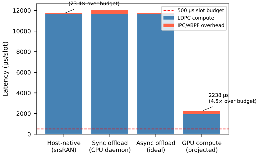
Per-slot latency breakdown (MCS28, 273 PRB, C=24 CBs)
