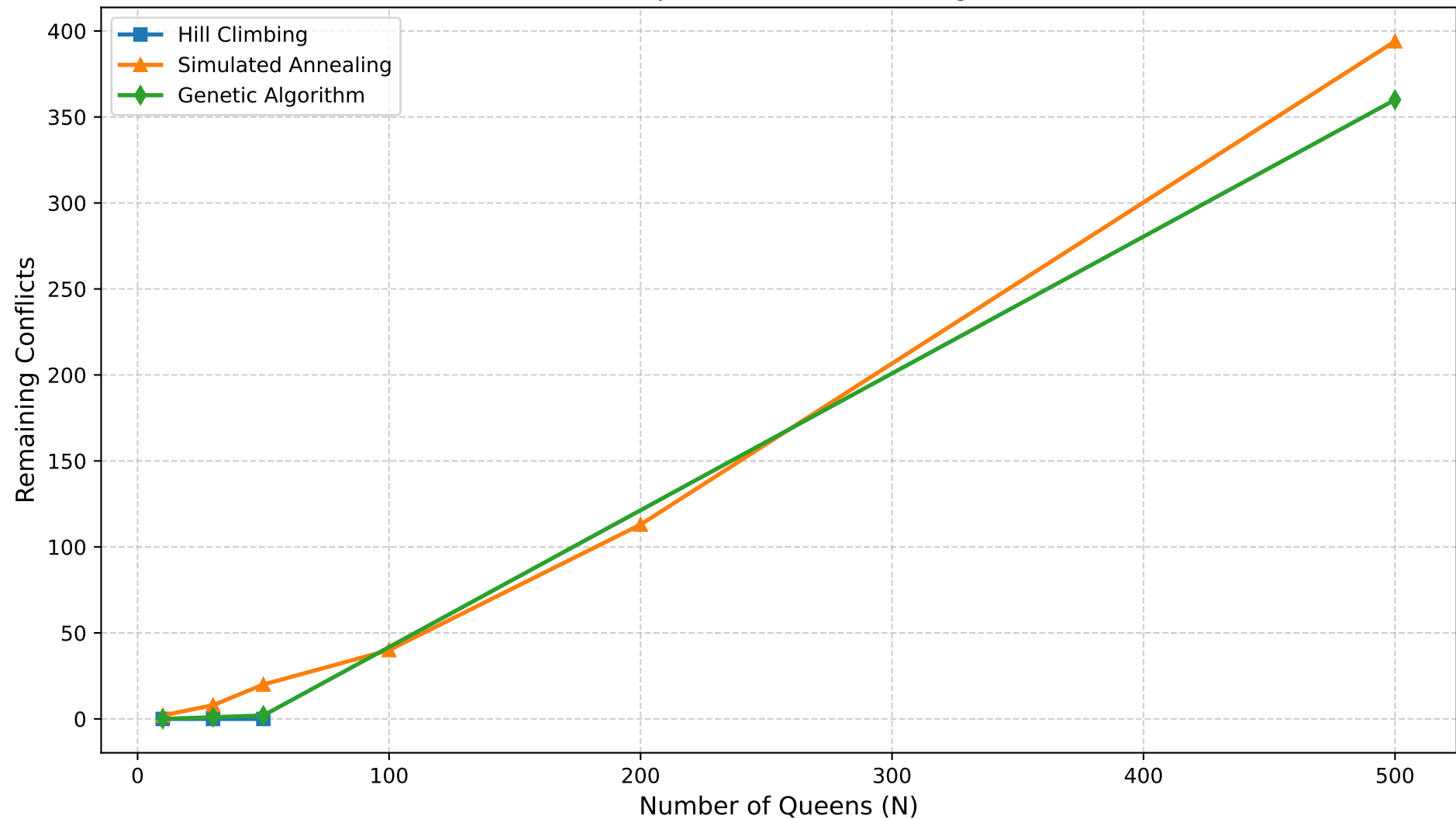
Conflict Comparison of Heuristic Algorithms
