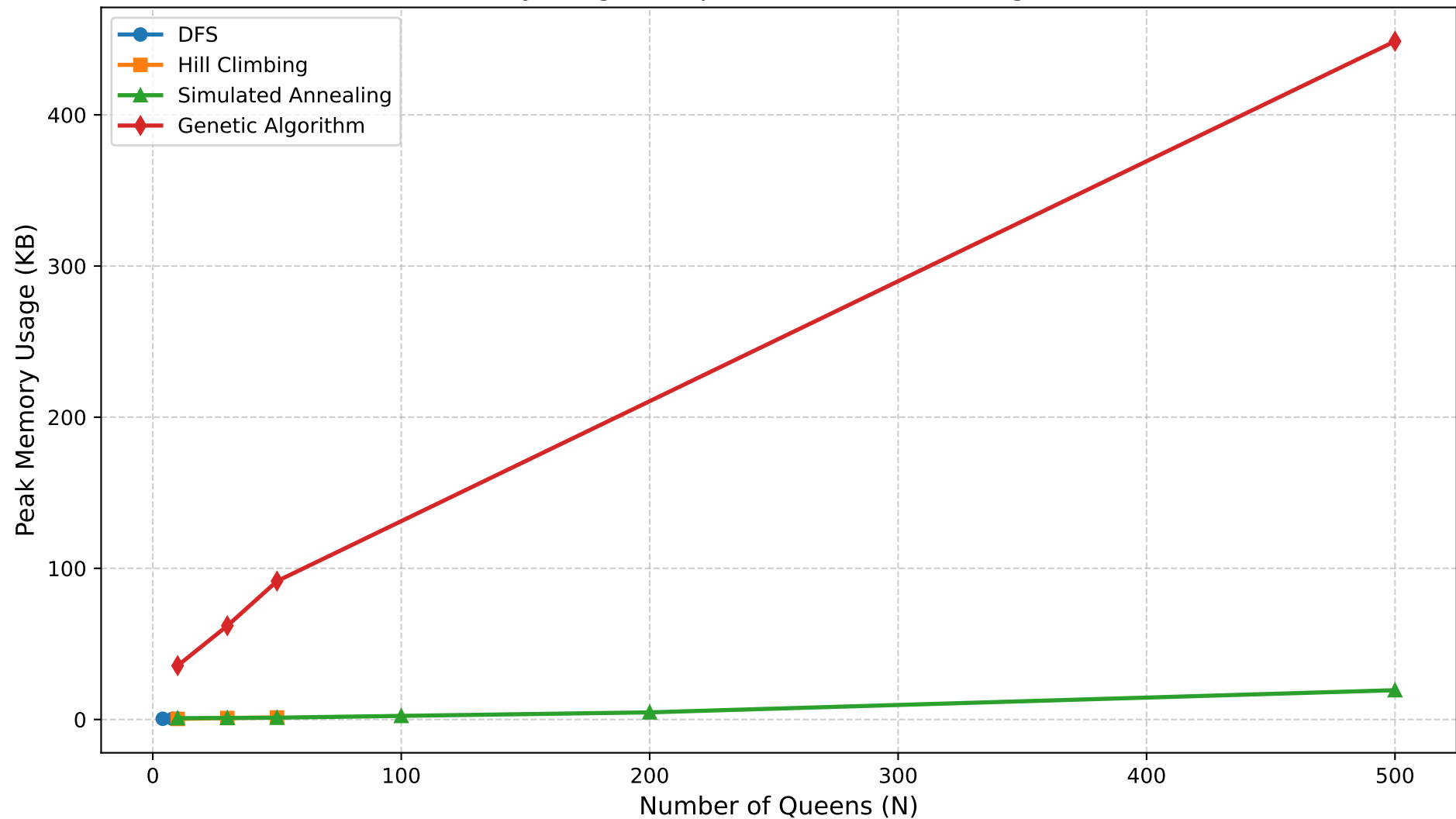
Memory Usage Comparison of N-Queens Algorithms
