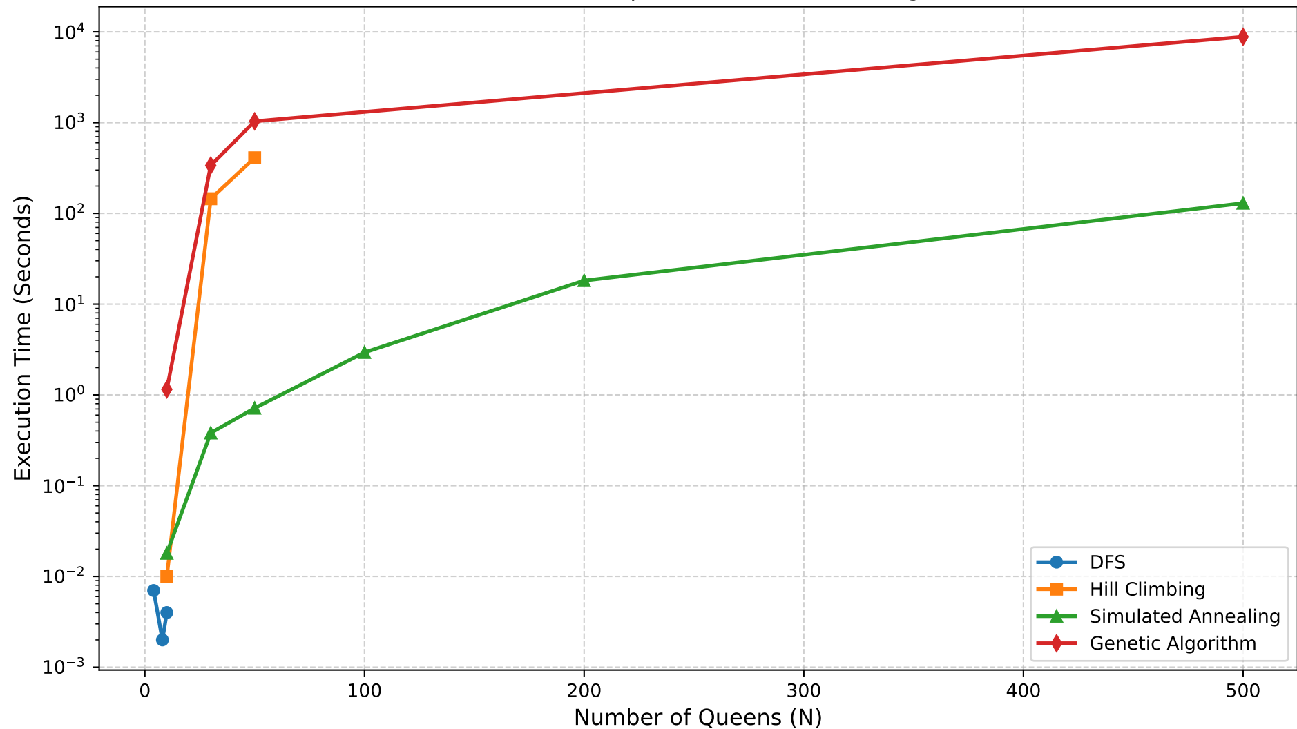
Execution Time Comparison of N-Queens Algorithms
