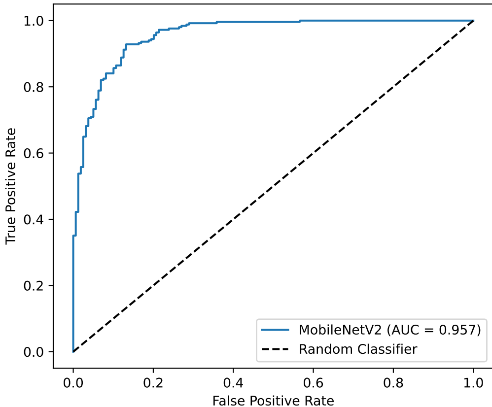
MobileNetV2 - ROC Curve
