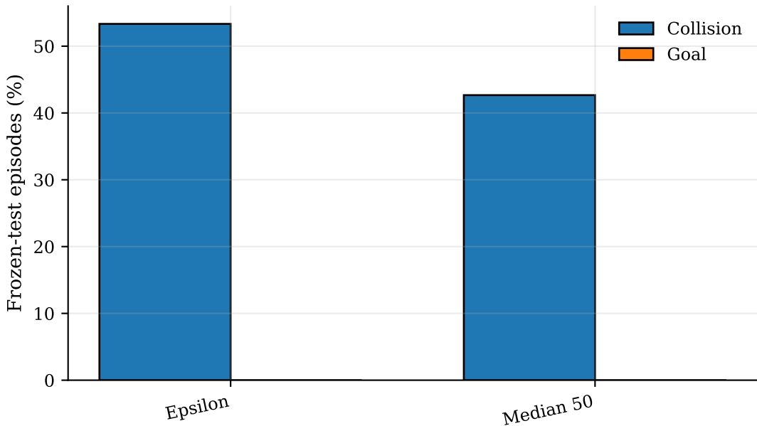
MetaDrive Collision and Goal Rates
