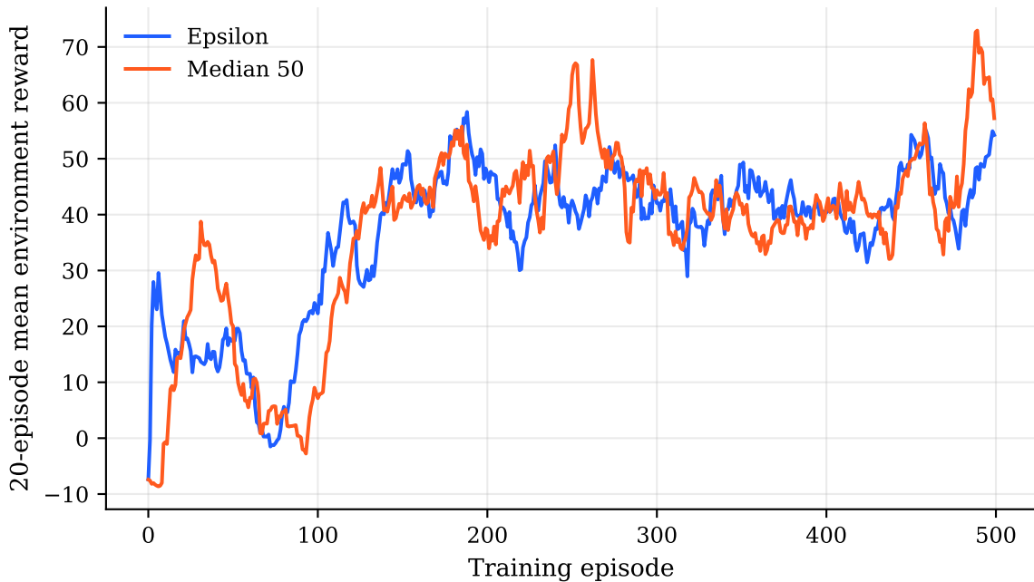
MetaDrive DQN Training Reward
