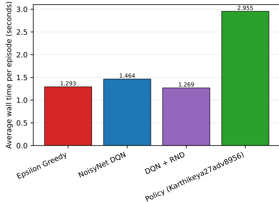
Train
