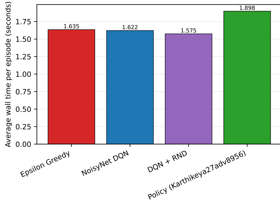
Frozen Test
