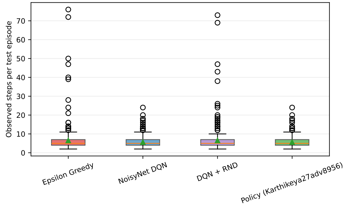
Frozen-Test Episode-Step Distribution
