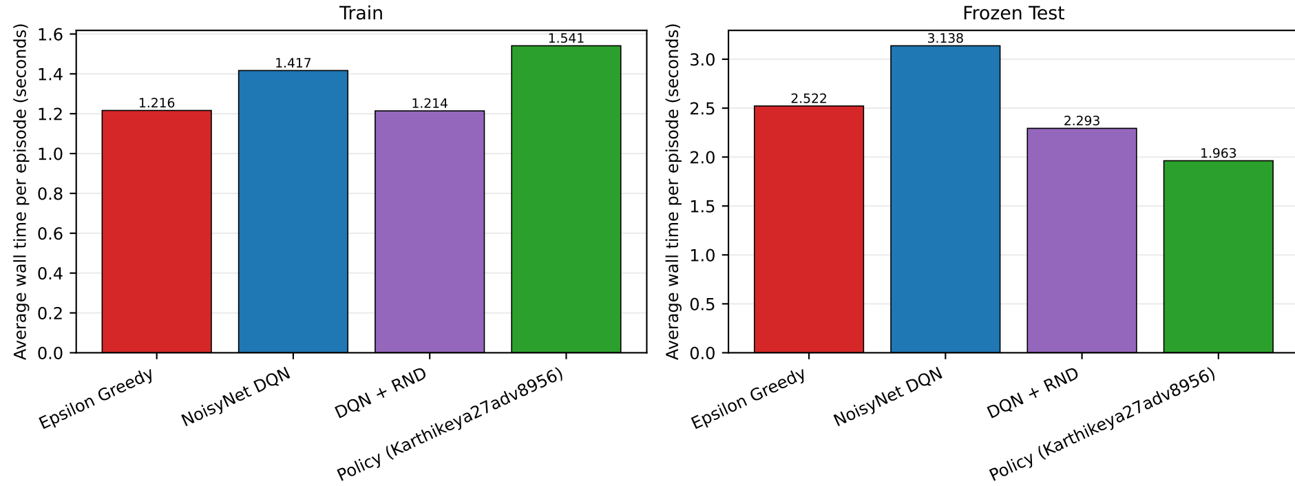
Average Training and Frozen-Test Episode Time
