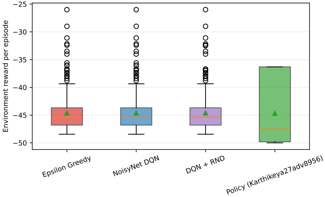
Frozen-Test Environment Reward Distribution
