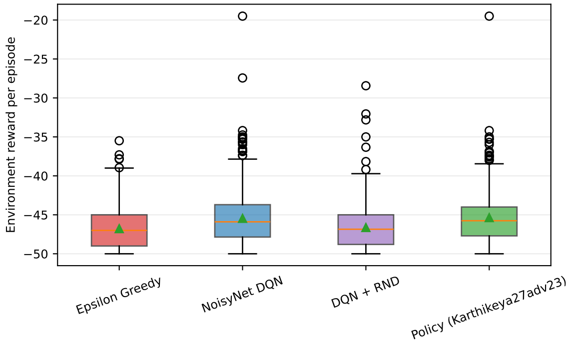
Training Environment Reward Distribution
