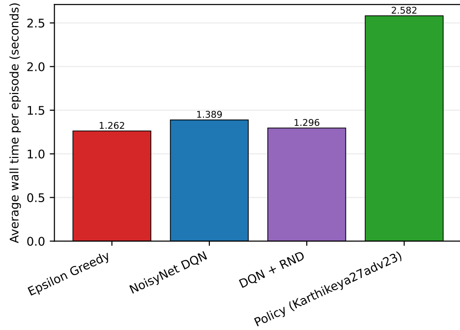
Train
