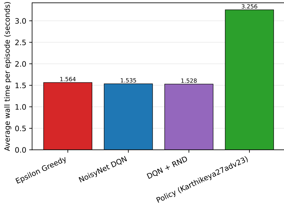
Frozen Test
