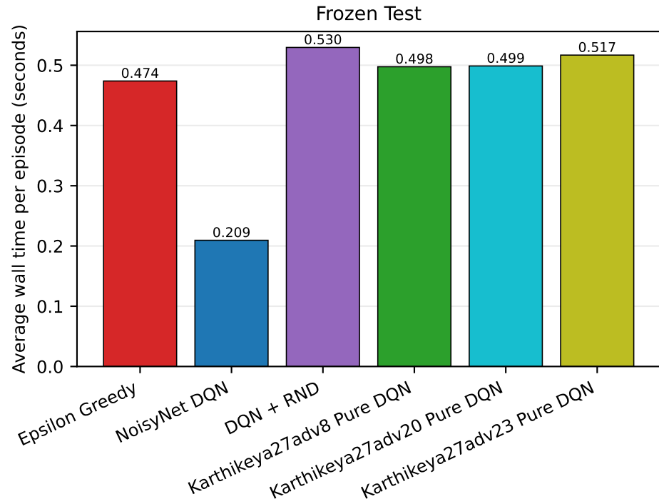
Average Training and Frozen-Test Episode Time
