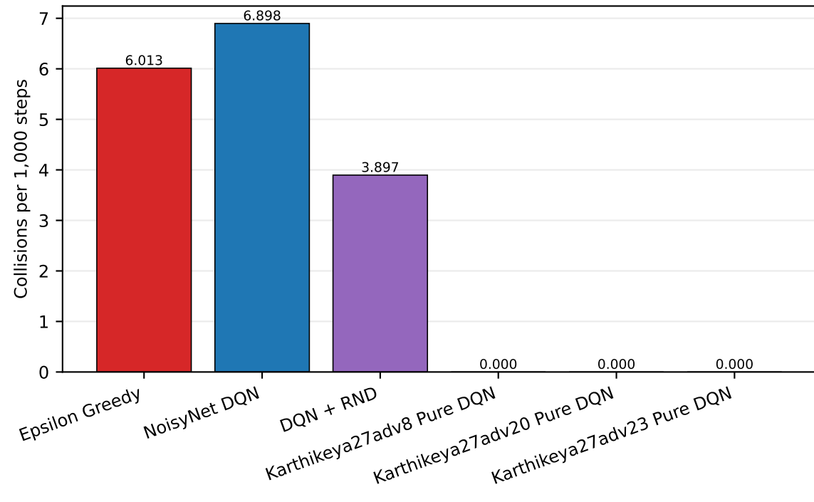
Frozen-Test Collisions per 1,000 Steps
