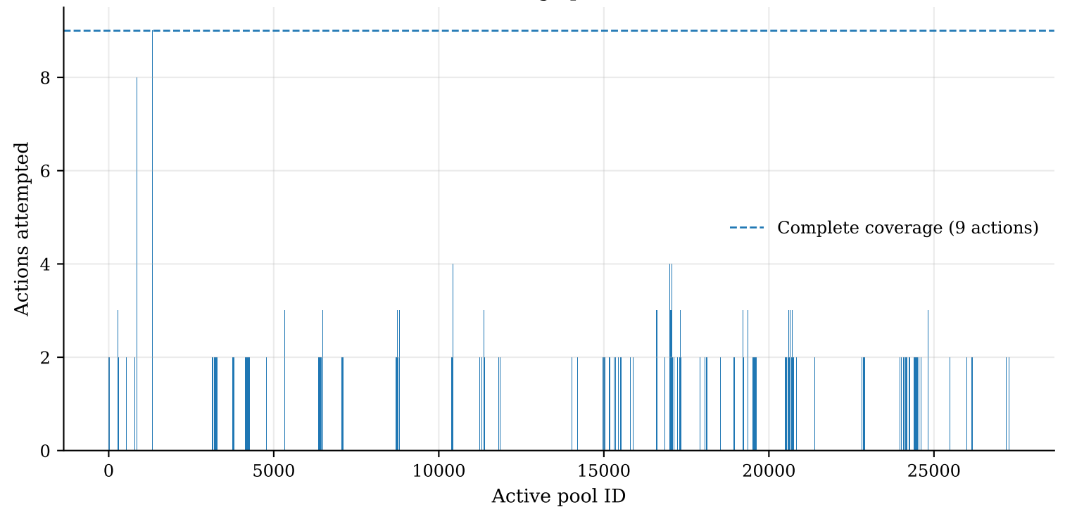
Action Coverage per Active Pool
