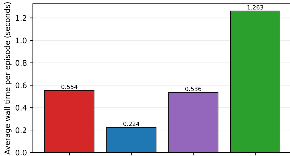
Frozen Test
