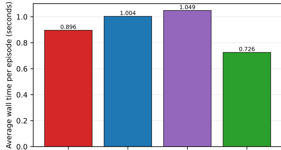
Train
