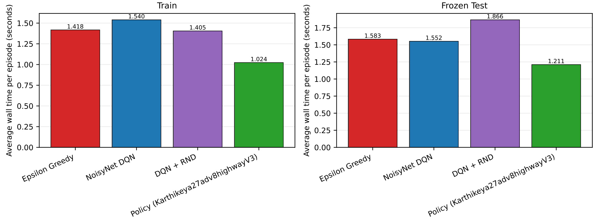
Average Training and Frozen-Test Episode Time
