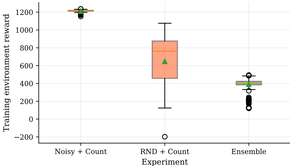
Training Reward Distribution Across All Episodes
