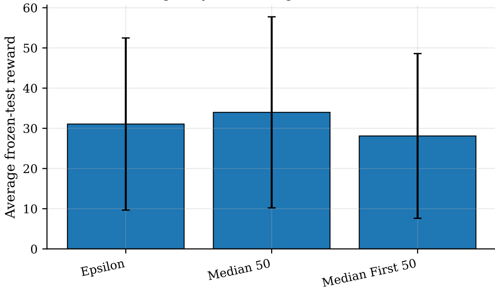
HighwayEnv Average Test Reward
