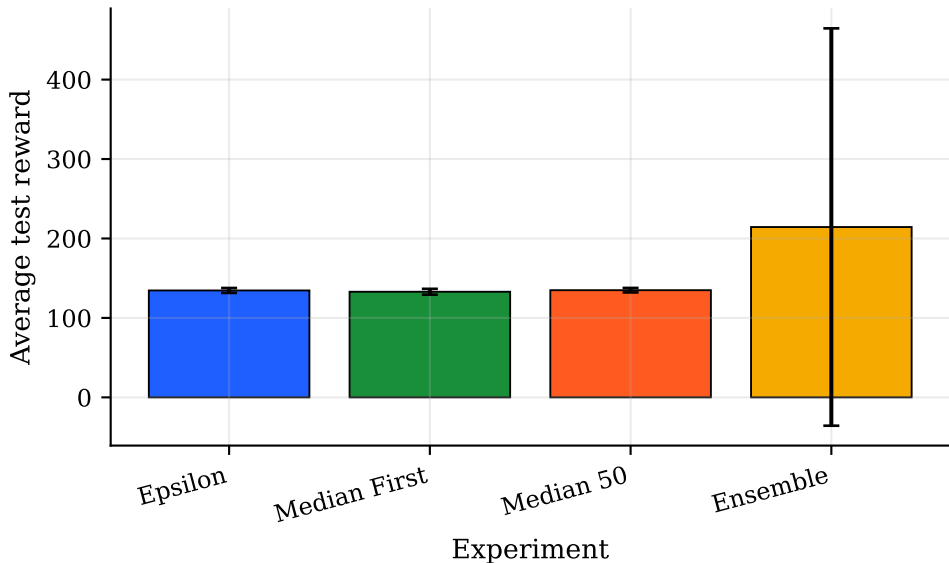
Average Test Reward Across All Test Episodes
