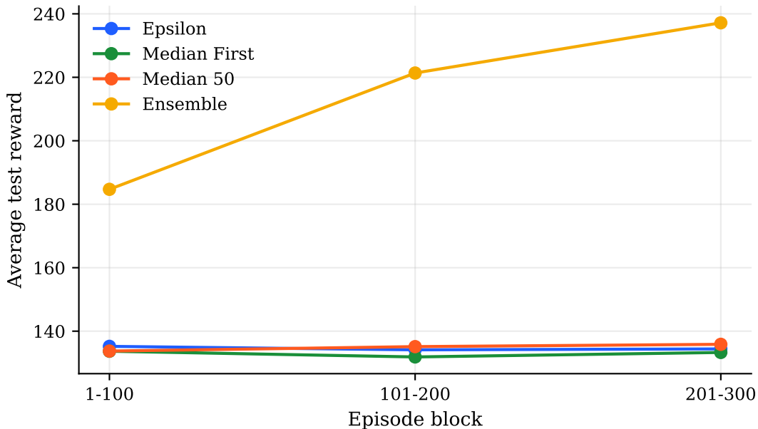
Testing Reward by Episode Block
