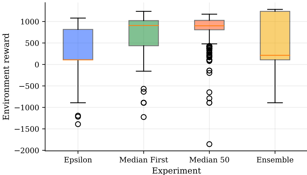
Test Reward Distribution Across All Test Episodes
