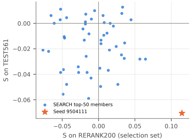
B Frozen top 50: RERANK \rightarrow TEST ( r = -0.15 )
