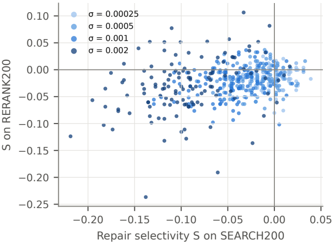
A 500 random audit candidates ( r = 0.32 ; within \sigma : 0.11, 0.17, 0.26, 0.31)
