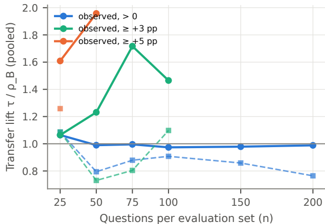
B Lift: observed (solid) vs item-fragility null (dashed)
