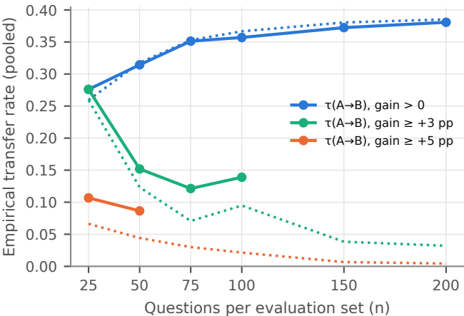
A P(\text{improver on B} \mid \text{improver on A}), 500 \text{ audit cand.} dotted: \rho_B (no-persistence reference)
