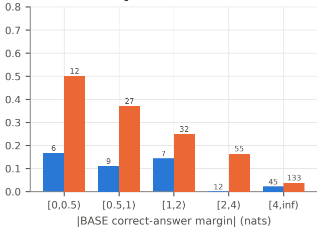
B BASE correct: regression rate
