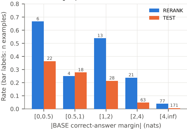
A BASE wrong: repair rate
