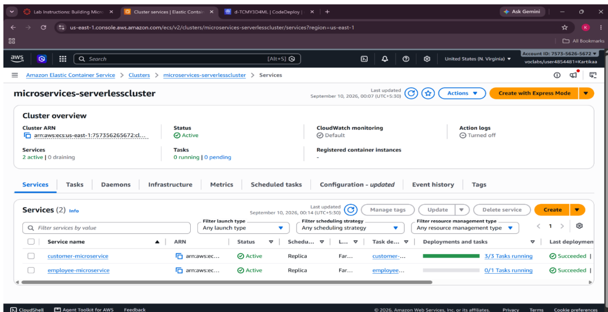
Figure 2: Amazon ECS cluster showing the Customer and Employee microservices in an active state.
