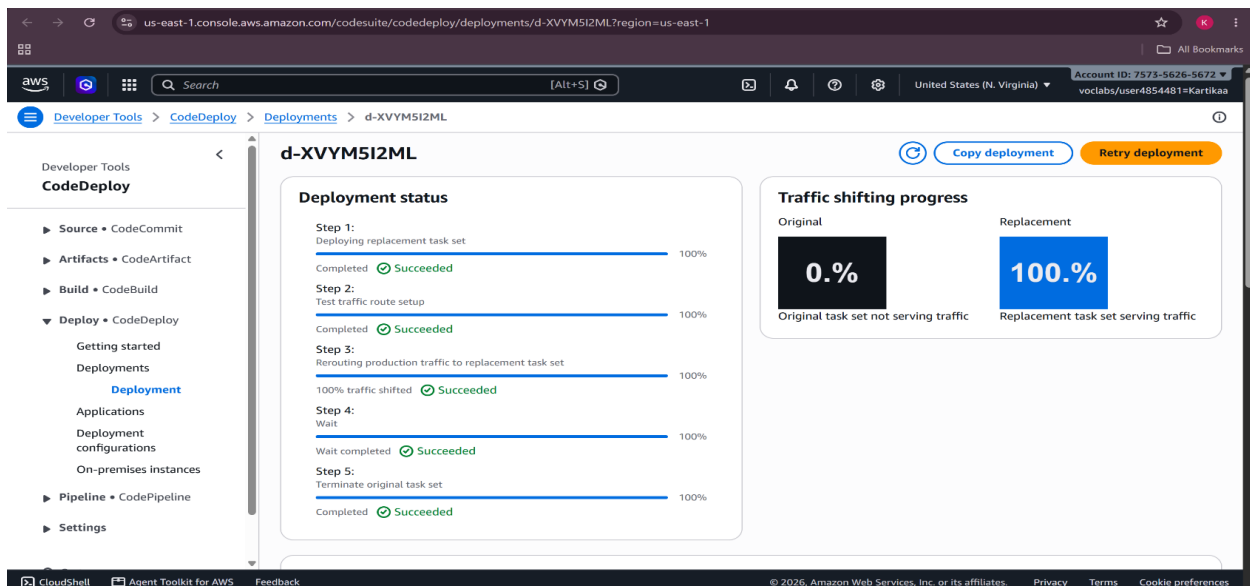
Figure 5: AWS CodeDeploy showing successful blue/green deployment with 100% of traffic shifted to the replacement task set.
