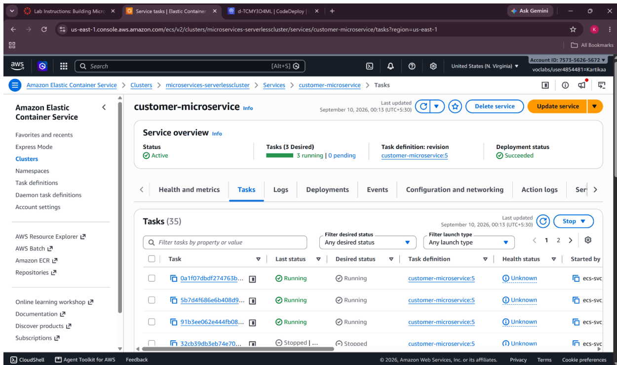
Figure 3: Customer Microservice showing running ECS tasks.
