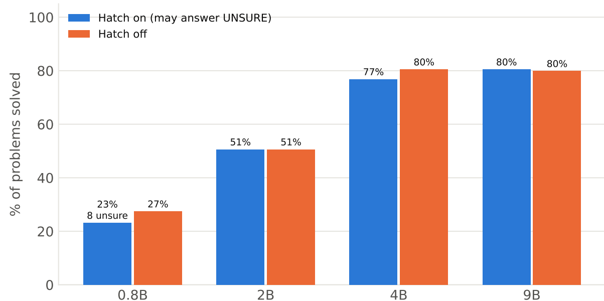
Qwen3.5 on humaneval+: offering an UNSURE option
