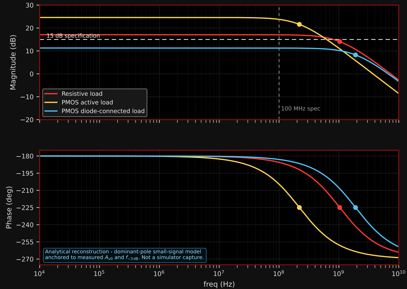
AC Response - comparison of the three CS amplifier load configurations
