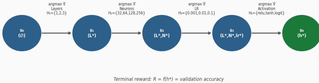
Figure 1. DP-HPO formulated as a finite-horizon MDP. Each stage commits one hyperparameter dimension via Bellman argmax.
