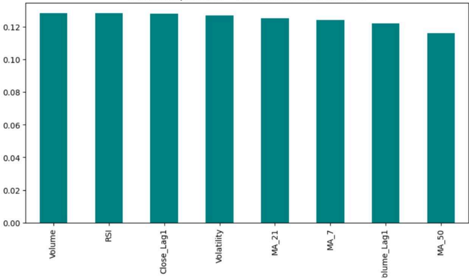
Feature Importance — AAPL Price Direction Model
