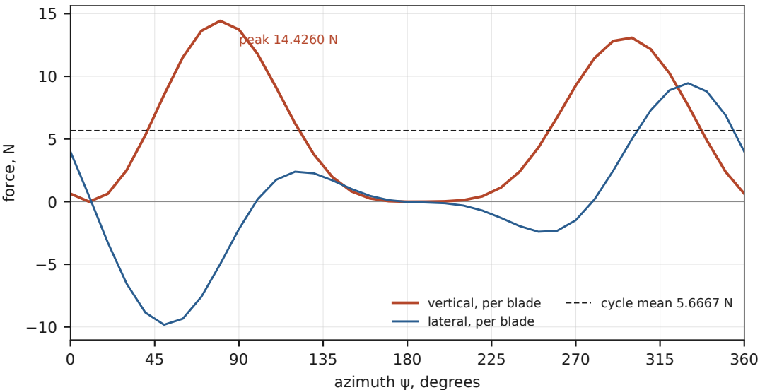
blade force through one revolution, peak to mean 2.5458
