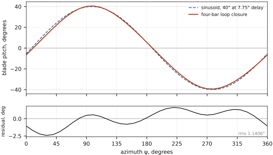
blade pitch against azimuth
