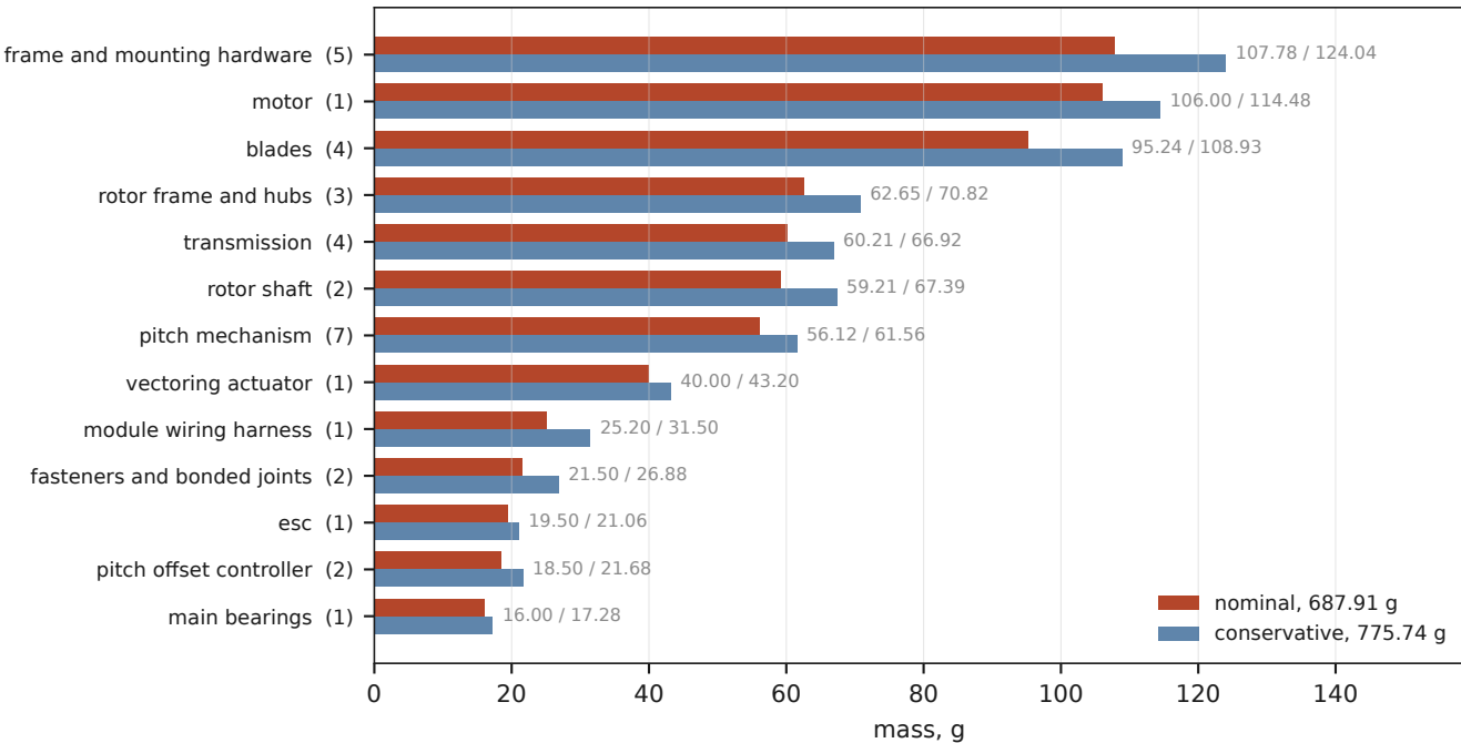
module mass by group, 34 drawn lines thrust to weight 2.5191 design, 2.1221 stacked
