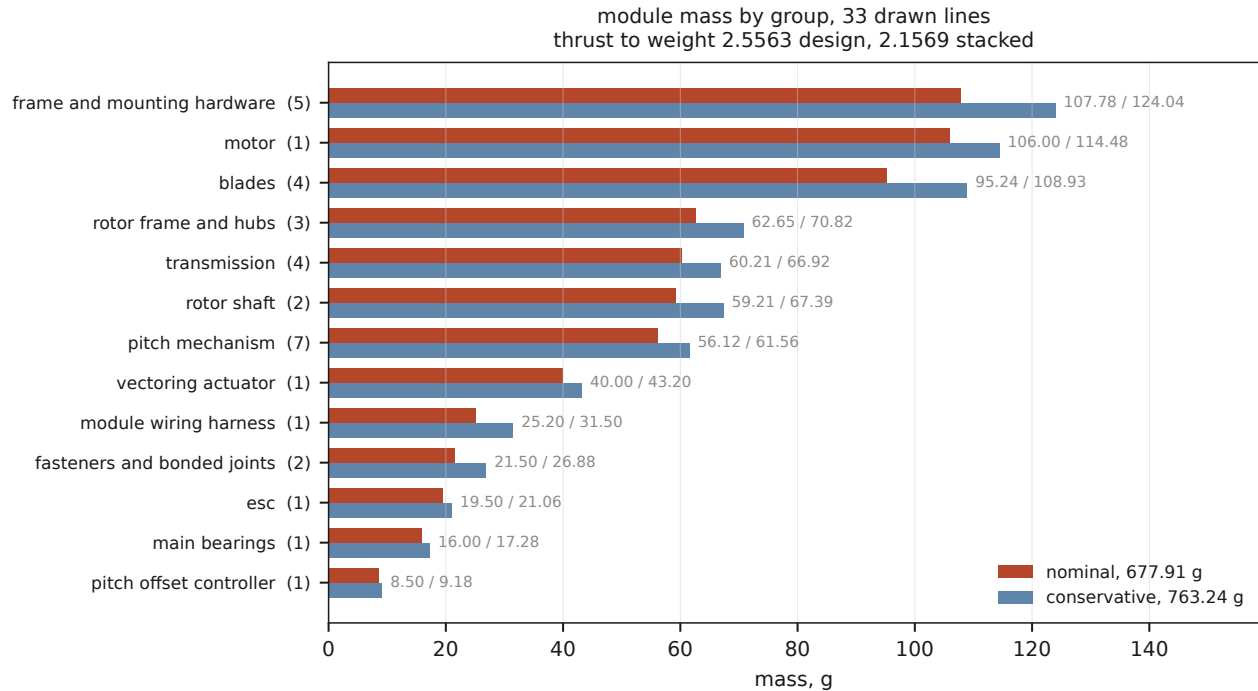
Figure 7: Module mass by group. 33 drawn lines totalling 677.91 g nominal and 763.24 g conservative, with the line count per group in brackets. Thrust to weight is 2.5563 at the design point and 2.1569 with the coefficient and mass downsides stacked.
