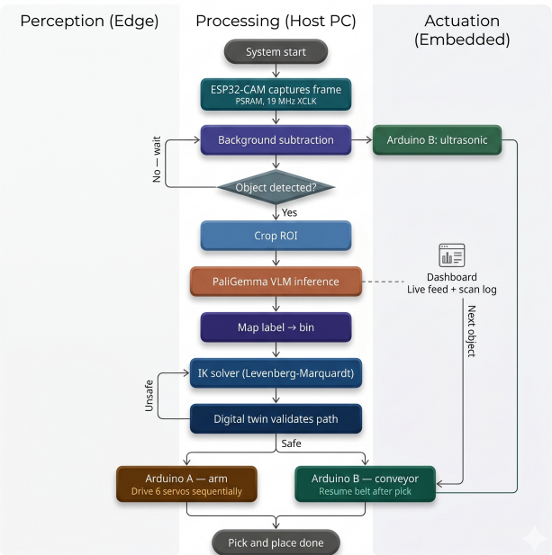
Figure 1. System Flowchart
