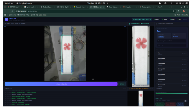
Figure 6. IndERA-Drishti Dashboard streaming the live conveyor feed and displaying live PaliGemma inference results (e.g., detecting a fan).
