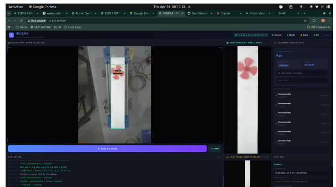
Figure 7. Dashboard view highlighting the bounding box overlay, extracted model input preview, and chronological scan history.
