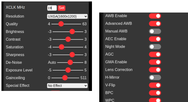
Figure 4. ESP32 OV3660 camera parameter configuration, showcasing the custom XCLK adjustments applied to stabilize the video feed
