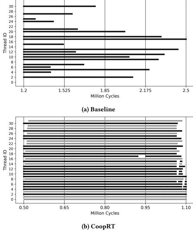
Figure 11: RT unit trace_ray instruction execution timelines. Dark and light gray bars represent active and originally inactive threads, respectively. A continuous bar indicates a non-empty traversal stack. bath scene, 256x256 resolution path tracing.
