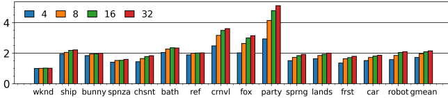
Figure 19: Speedups of CoopRT for subwarp sizes of 4, 8, 16 and 32 normalized to baseline.
