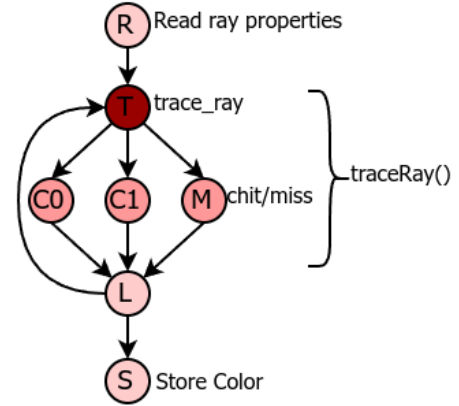
Figure 5: A Simplified Control Flow Diagram of Listing 1. C0, C1 are closest-hit shaders, and M is a miss shader. L is the loop iteration block.
