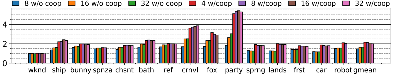
Figure 13: Normalized speedups for different RT warp buffer sizes with and w/o CoopRT. Baseline is 4-entry warp buffer without CoopRT. 1 warp per thread block, 32 thread blocks in one SM at a time. Missing data points are due to consistently crashing or timing out simulations.
