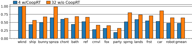
Figure 14: Latency of the slowest warps, normalized to baseline (4 buffer entries without CoopRT). Lower the better.
