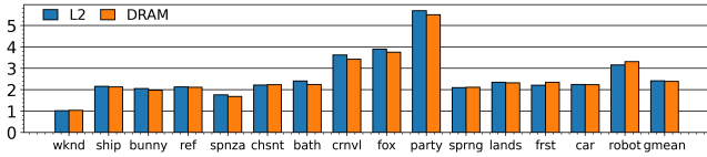
Figure 12: Normalized L2 ↔ Interconnect, and DRAM bandwidth with CoopRT over the baseline.
