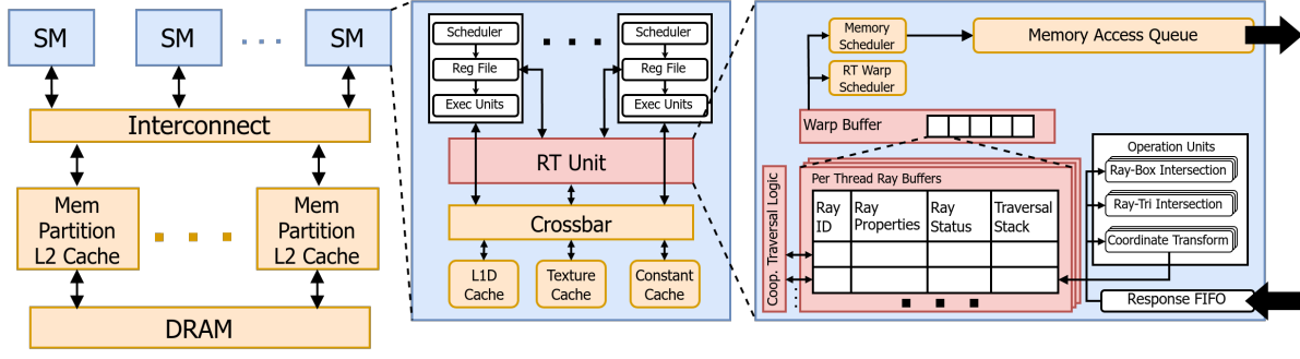
Figure 3: Diagram of the GPU model used in this study. Red blocks indicate the modified components. Redrawn from [37].
