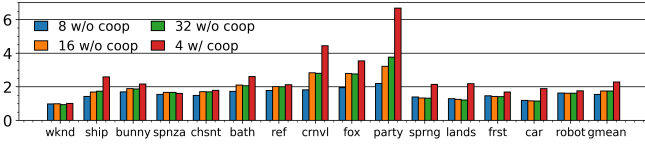
Figure 15: Normalized improvement in EDP for different RT warp buffer sizes. Baseline is 4-entry warp buffer without CoopRT.
