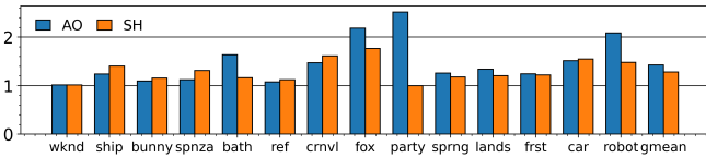
Figure 17: Speedups of CoopRT for AO and SH shaders normalized to baseline.
