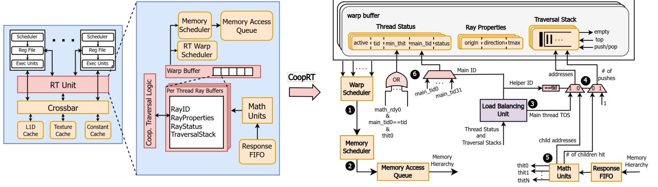
Figure 7: Overview of the modified RT unit. Orange blocks indicate existing hardware, red blocks are newly added per-thread structures, and purple blocks are newly added per-RT unit (therefore per-SM) structures. main_tid is a new 5-bit field added to Thread Status in the warp buffer.
