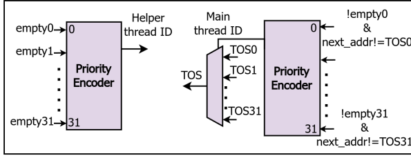
Figure 8: Load Balancing Unit.
