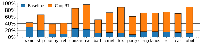
Figure 10: Average thread utilization.
