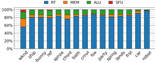
Figure 1: Pipeline stalls from different instructions, RT: trace_ray instructions, MEM: load/store instructions from CUDA cores, ALU: compute instructions from CUDA cores, SFU: special function instructions from CUDA cores. Configuration: 256x256 resolution, path tracing, 1 sample-per-pixel.
