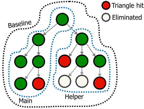
Figure 6: Example BVH tree traversal comparing baseline and cooperative traversal.
