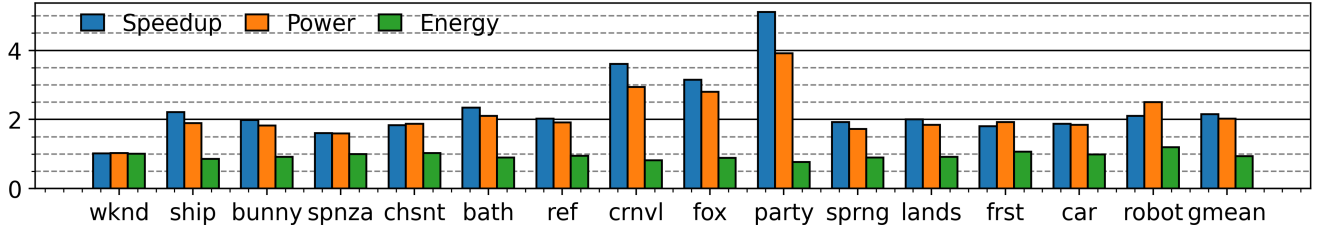
Figure 9: Normalized speedup, power and energy consumptions of CoopRT over the baseline RT unit.
