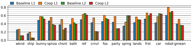
Figure 16: L1 and L2 cache miss rates.
