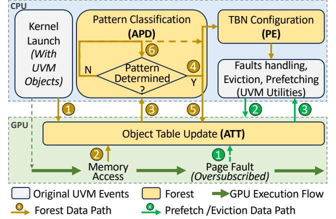
Figure 11: Workflow of Forest.
