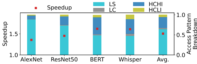
Figure 20: Speedup and access pattern breakdown of SpecForest on real-world DL workloads.
