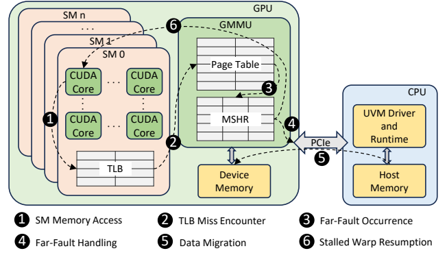
Figure 2: UVM walkthrough for far-faults.
