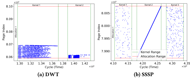
Figure 8: Memory access patterns of DWT and SSSP.
