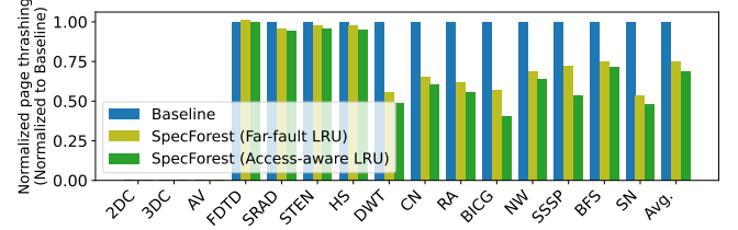
Figure 14: Page thrashing normalized by Baseline.
