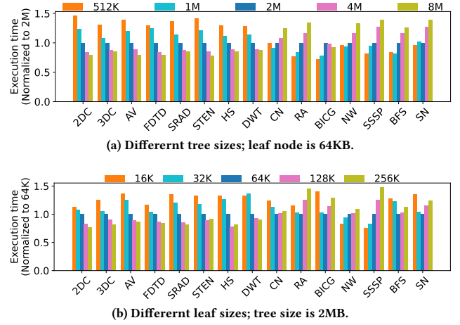
Figure 4: Execution time with diverse tree configurations (lower is better).
