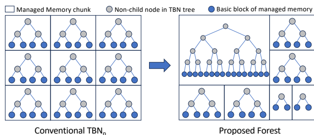
Figure 1: TBNp vs. Forest: TBNp uses homogeneous tree prefetchers for all memory blocks while Forest flexibly applies heterogeneous trees to support diverse access patterns.
