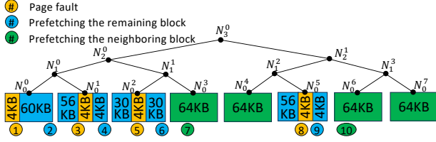
Figure 3: TBNp operations. For simplicity, this example denotes 512 KB of consecutive memory, while each TBN tree represents a 2 MB VABlock in the original TBNp.
