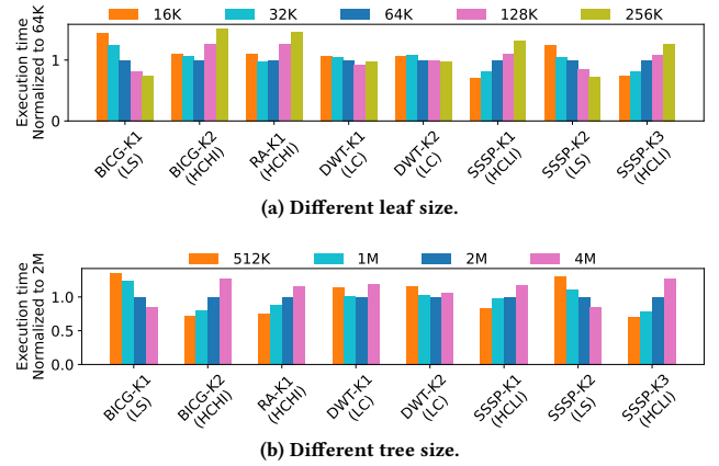
Figure 9: Performance impact of tree configurations for different access patterns (lower is better).
