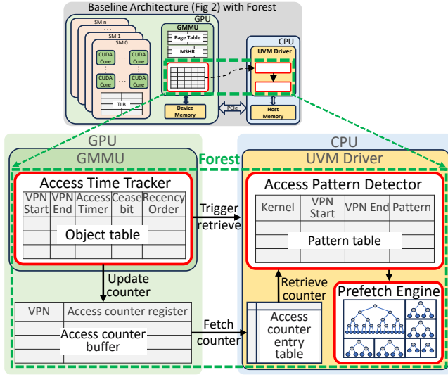
Figure 7: Architectural design of Forest (Newly added or modified components are highlighted with red outlines).
