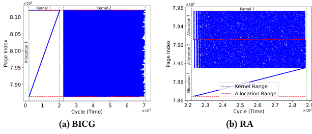
Figure 5: Memory access patterns of BICG and RA.
