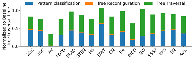
Figure 21: Runtime overhead breakdown. (Normalized to the Baseline TBNp tree traversal time)
