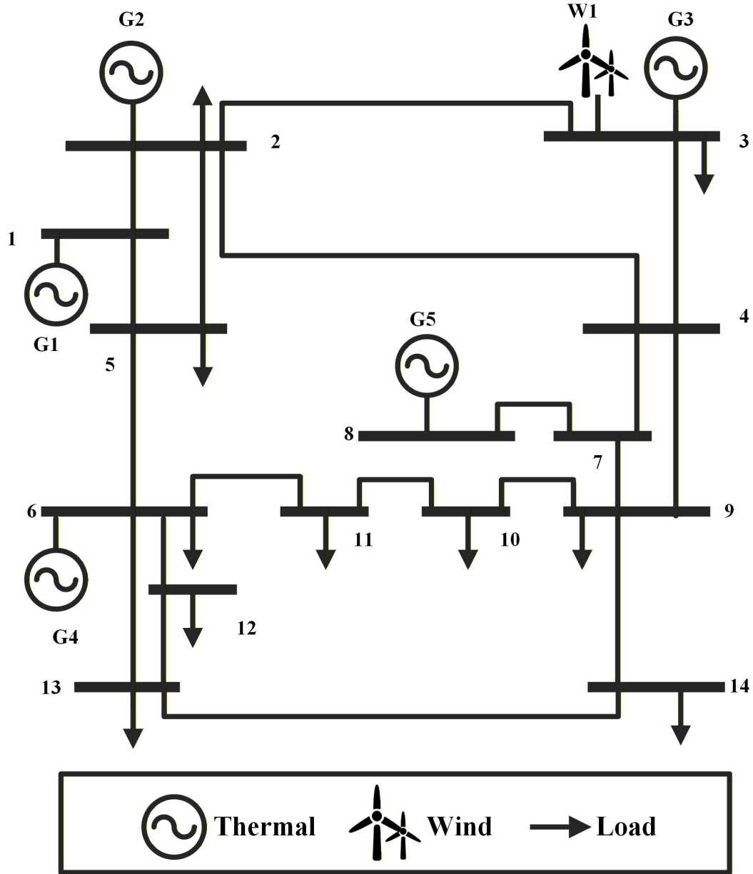
Fig. S1. Topology of the modified IEEE 14-bus test system.
