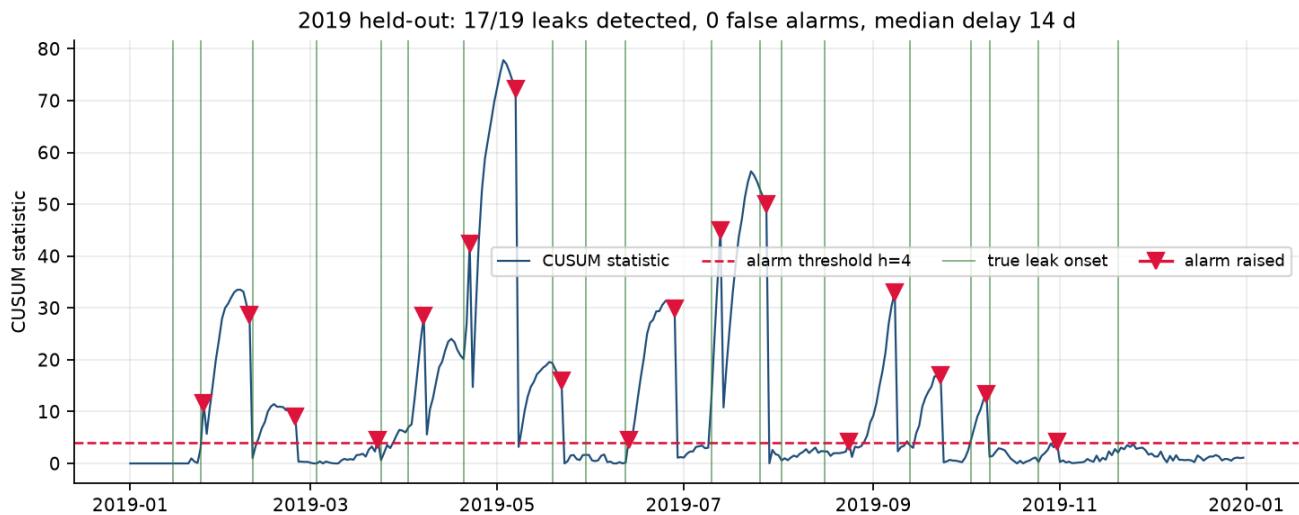
Figure 4. The detector running across the held-out year. The blue line is accumulated evidence, the dashed red line the alarm threshold, green lines the true leak onsets and red triangles the alarms raised. Every alarm follows a genuine onset, and no alarm appears anywhere else.
