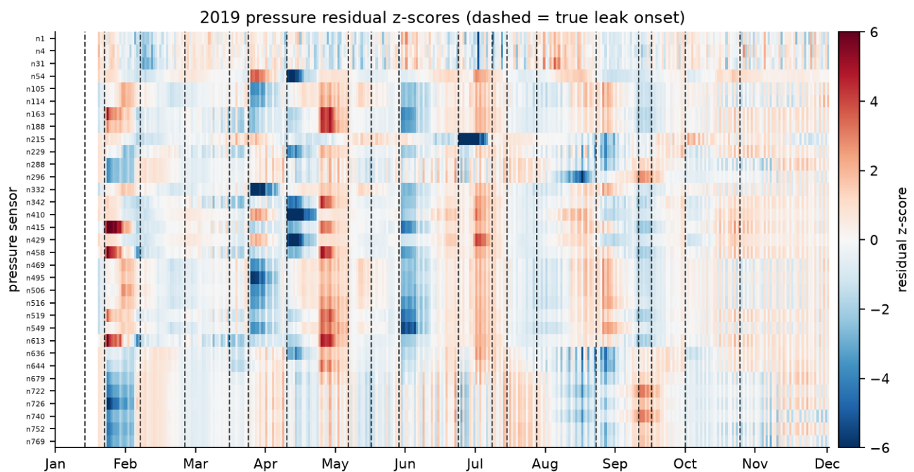
Figure 3. Residuals for all 33 sensors across 2019, expressed as z-scores. Each row is a sensor, each column a day. Dashed lines mark true leak onsets. Coloured bands appearing and persisting after a dashed line are leaks making themselves visible.
