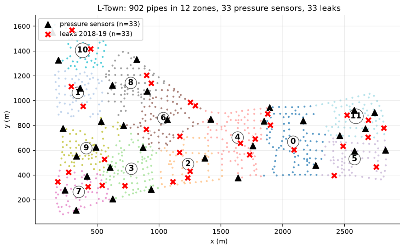
Figure 1. The L-Town network. Coloured dots are pipes, shaded by district. Black triangles are the 33 pressure sensors - the only inputs the system gets. Red crosses mark the 33 real leaks. Note how sparse the sensors are relative to the pipes: that sparsity is the core difficulty of the problem.
