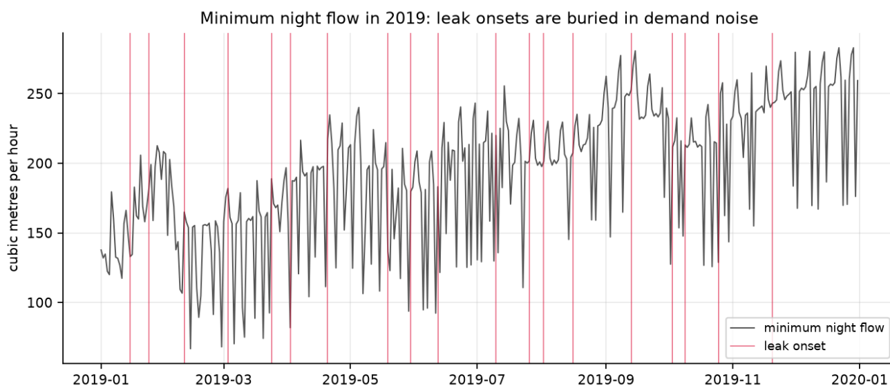
Figure 2. Night-time inflow through 2019. Each red line is a real leak starting. The onsets are indistinguishable from ordinary fluctuation - which is precisely why a better method is needed.
