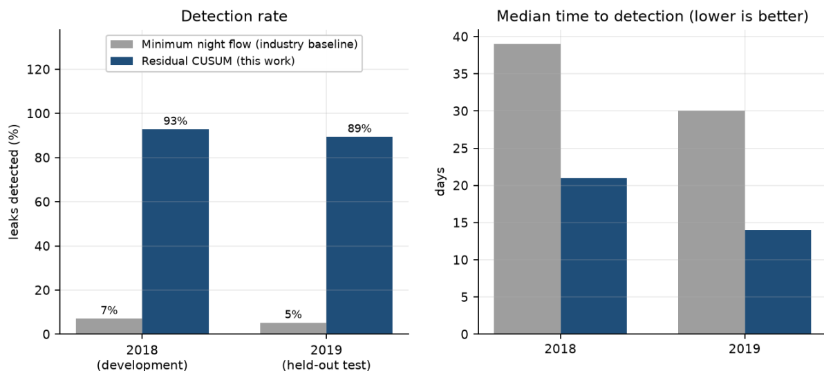
Figure 7. This method against minimum night flow, on both years.
