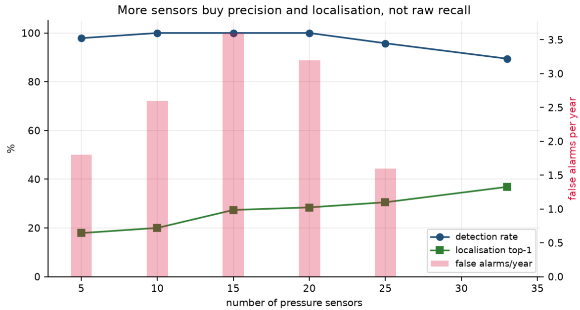
Figure 9. Detection, localisation and false alarms as the number of sensors varies. Sensors buy precision and location, not raw recall.
