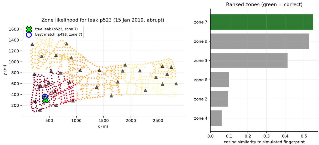
Figure 6. Leak p523 being localised. Left: every pipe shaded by how likely its district is, with the true leak marked in green and the best-matching pipe circled. Right: the districts ranked by score, the correct one shown in green.
