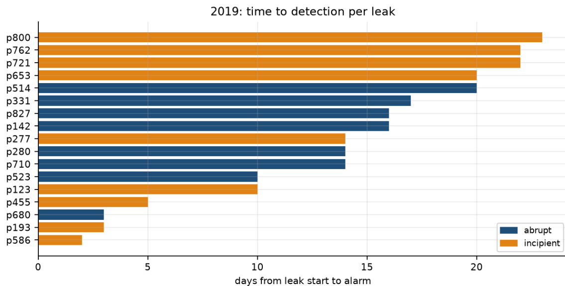
Figure 8. Time from leak start to alarm, leak by leak. Abrupt bursts (blue) are generally caught faster than slow incipient cracks (orange).
