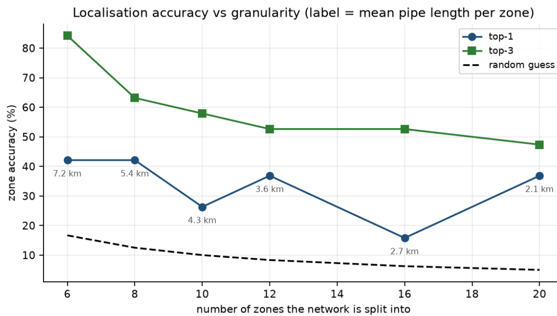
Figure 10. Accuracy against how finely the network is divided.
