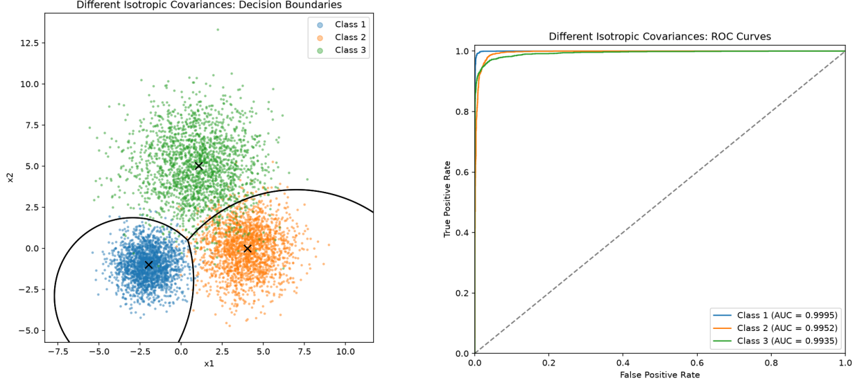
Figure 2: Test data, decision boundary, and one-vs-rest ROC curves. Accuracy: 96.57%.
