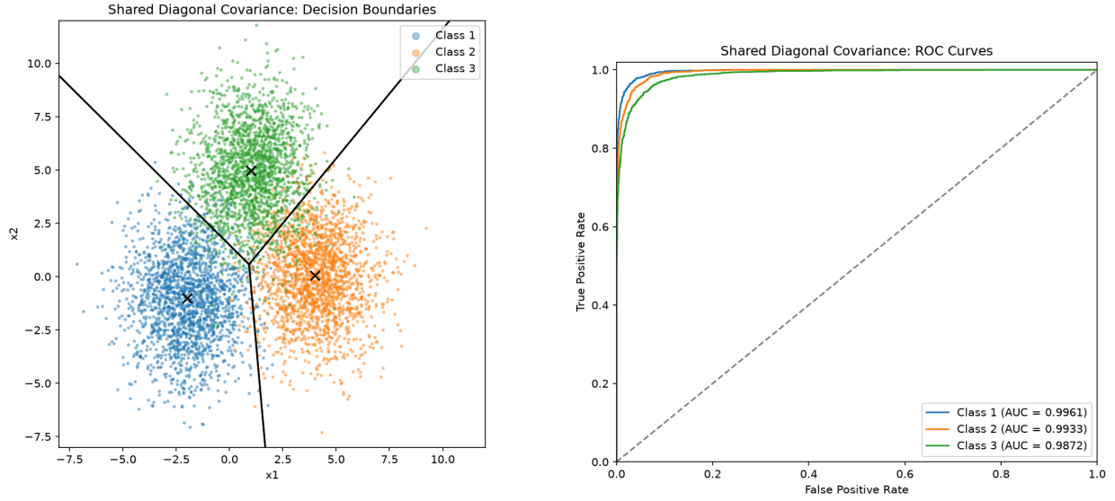
Figure 3: Test data, decision boundary, and one-vs-rest ROC curves. Accuracy: 93.65%.
