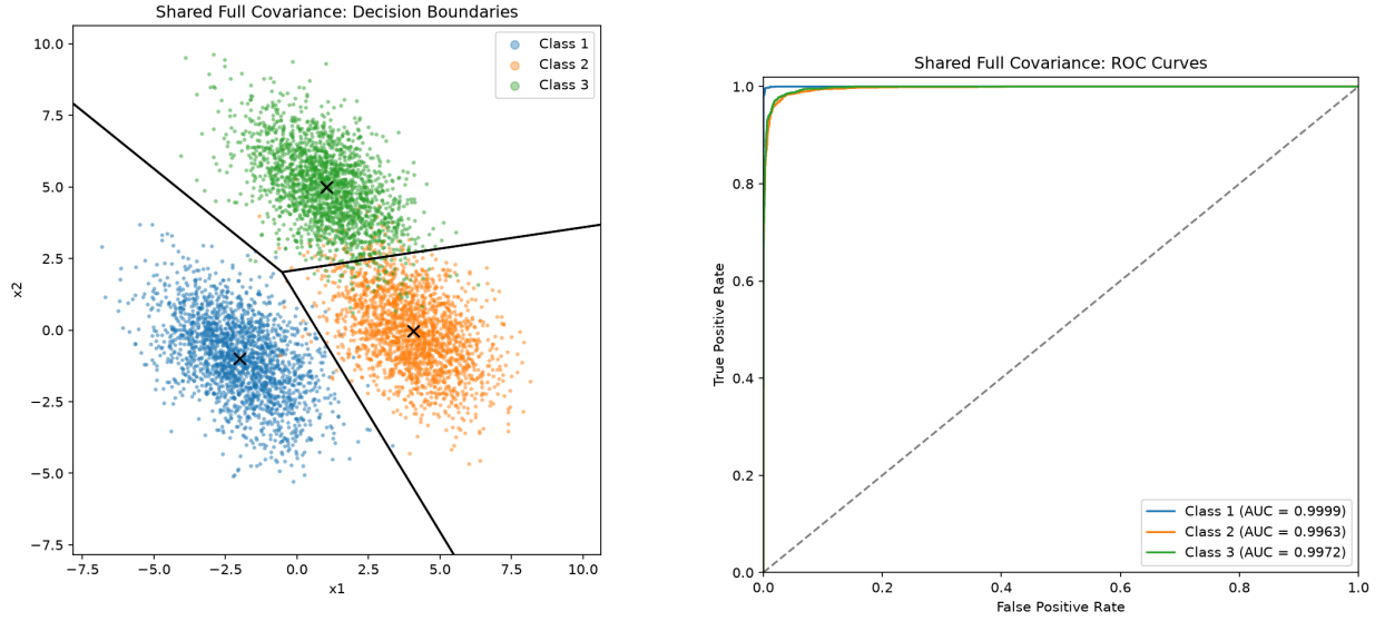
Figure 5: Test data, decision boundary, and one-vs-rest ROC curves. Accuracy: 97.40%.
