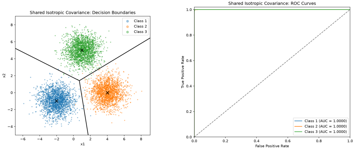
Figure 1: Test data, decision boundary, and one-vs-rest ROC curves. Accuracy: 99.73%.
