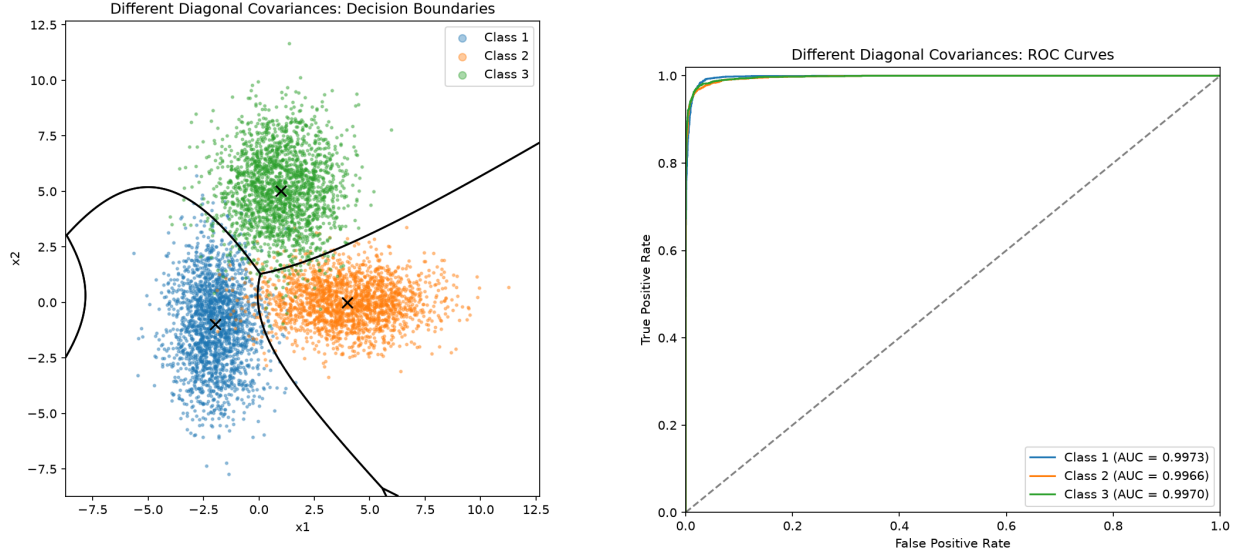
Figure 4: Test data, decision boundary, and one-vs-rest ROC curves. Accuracy: 96.40%.
