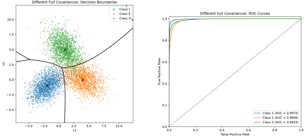
Figure 6: Test data, decision boundary, and one-vs-rest ROC curves. Accuracy: 95.03%.
