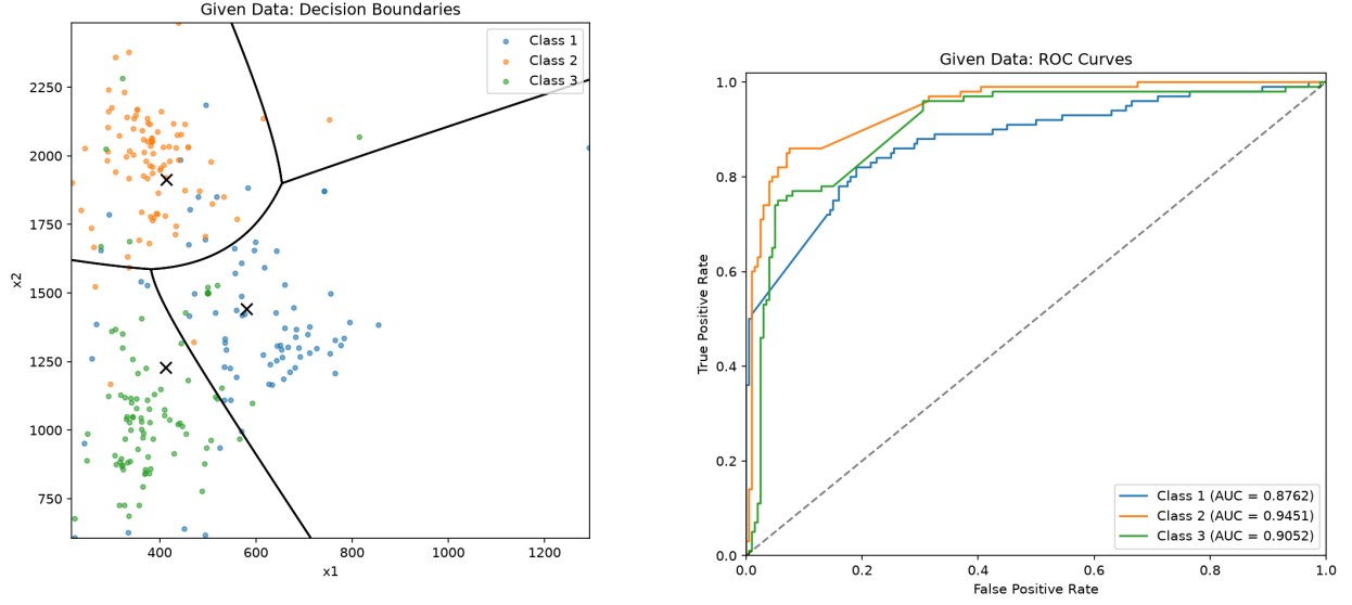
Figure 7: Test data, decision boundary, and one-vs-rest ROC curves. Accuracy: 80.00%.
