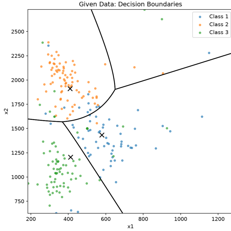
Figure 7: Test data and decision boundary. Accuracy: 78.89%.
