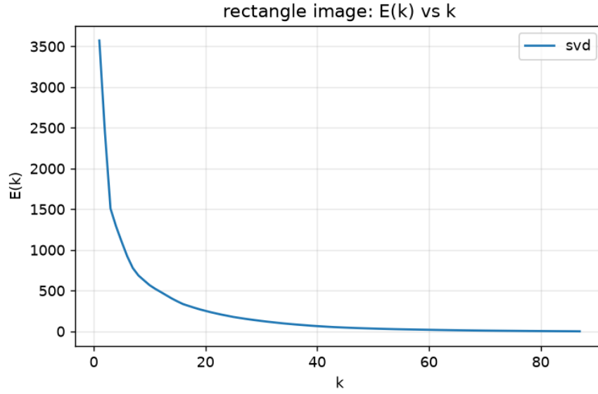
Figure 10: E(k) vs k , rectangular image, all k from 1 to 87.
