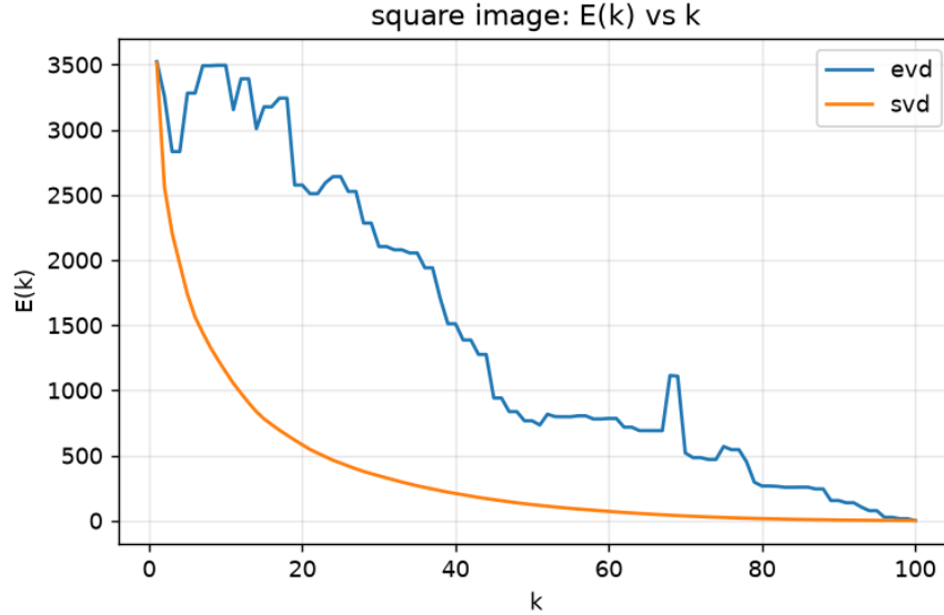
Figure 5: E(k) vs k , square image, all k from 1 to 100.
