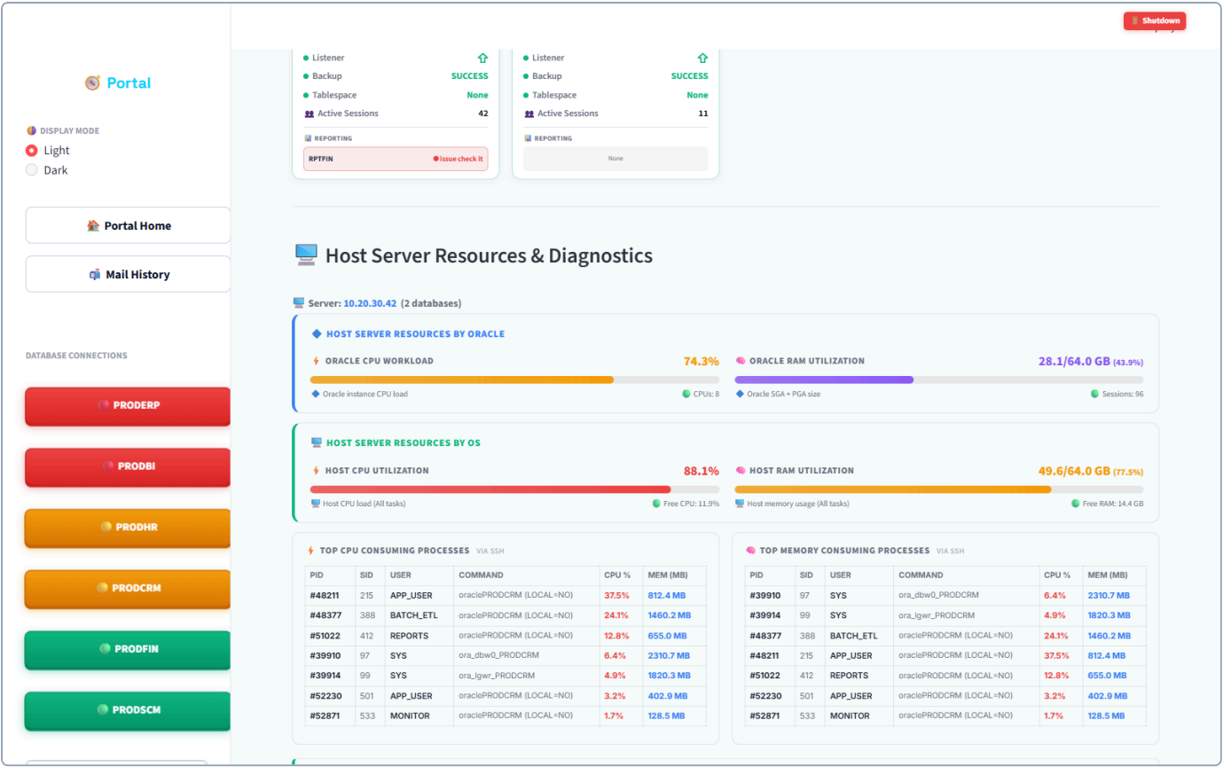
Figure 7: Host section – Oracle and OS resource cards (demo data)
