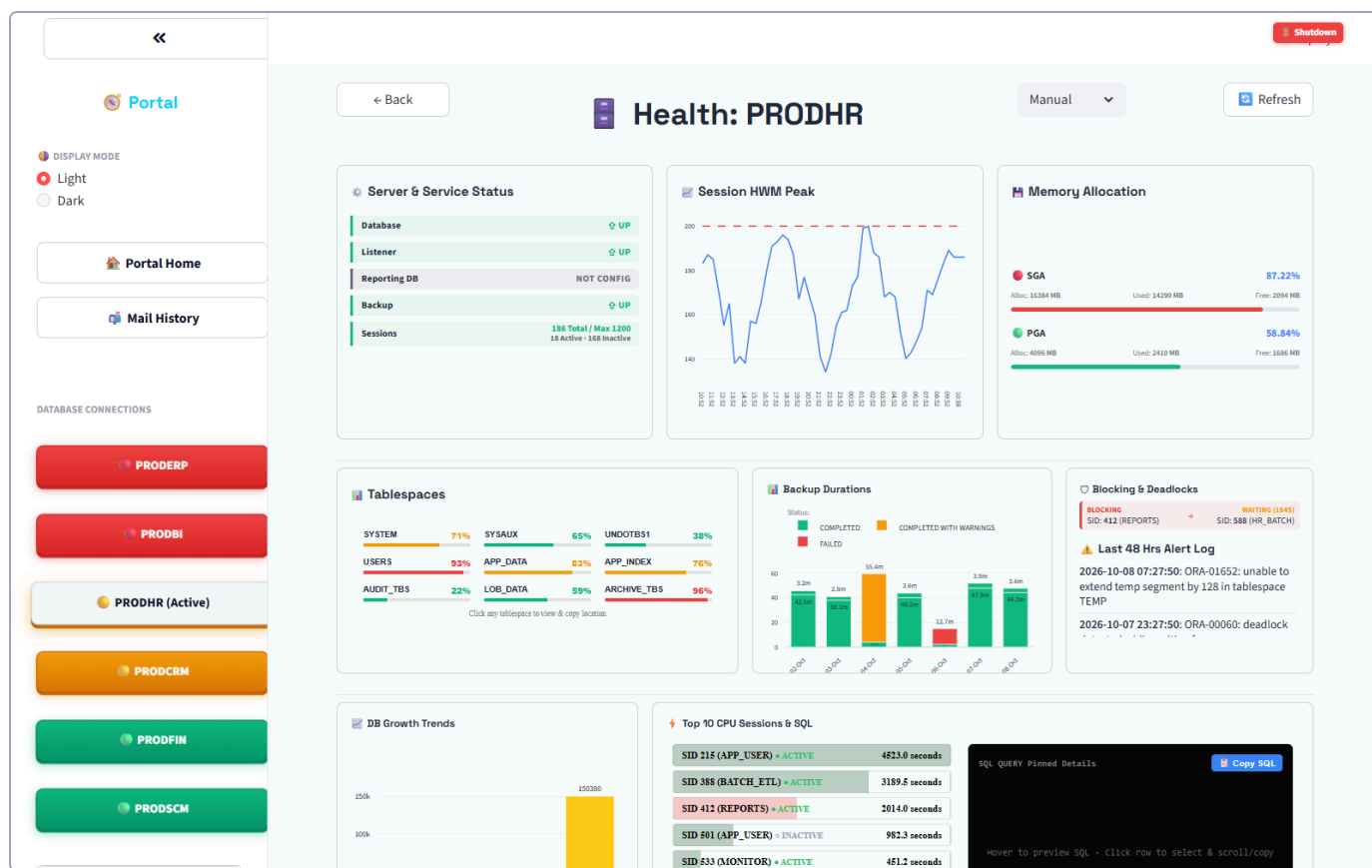
Figure 9: Health: PRODHR – status, sessions, memory, tablespaces, backups and blocking (demo data)
