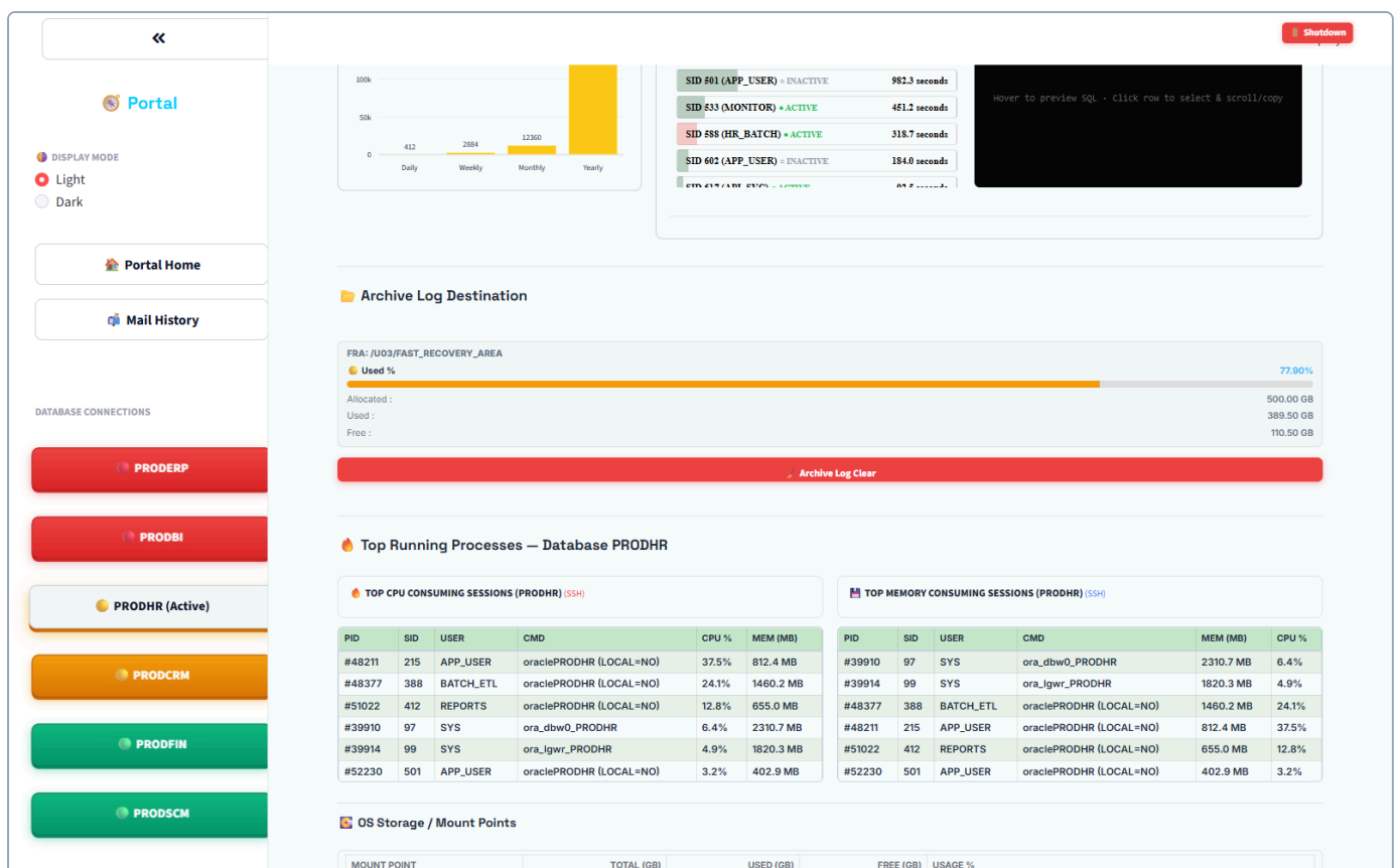
Figure 10: Growth trends, top CPU sessions and archive log destination (demo data)
