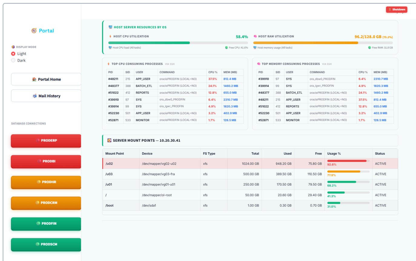
Figure 8: Top processes and server mount points for host 10.20.30.41 (demo data)
