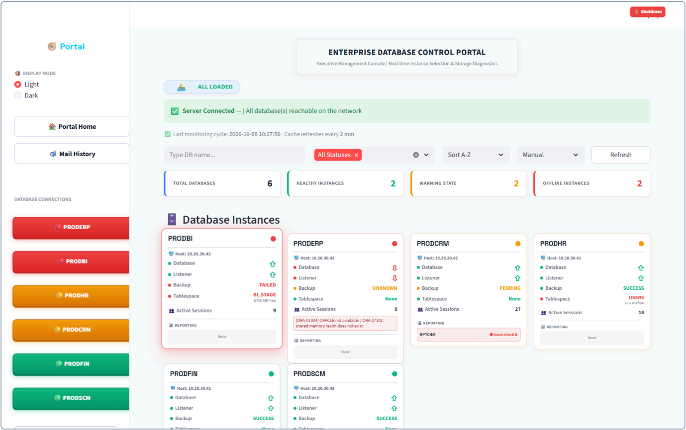
Figure 6: Cards for Critical (PRODBI, PRODERP), Warning (PRODCRM, PRODHR) and Healthy databases (demo data)
