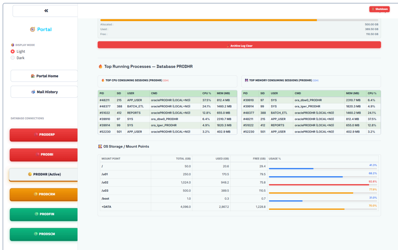
Figure 11: Top running processes and OS storage / mount points (demo data)
