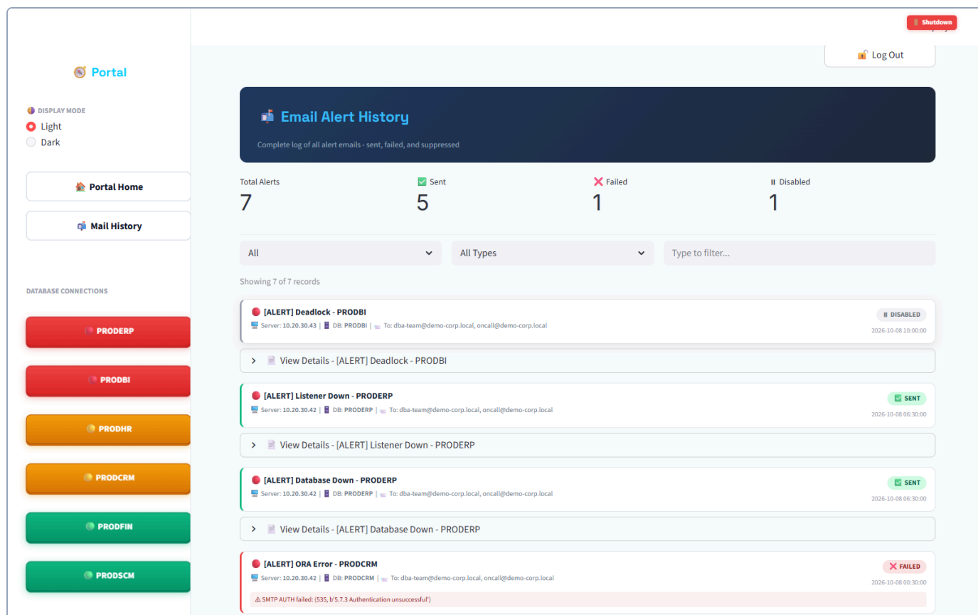
Figure 15: Email Alert History with sent, failed and disabled alerts (demo data)
