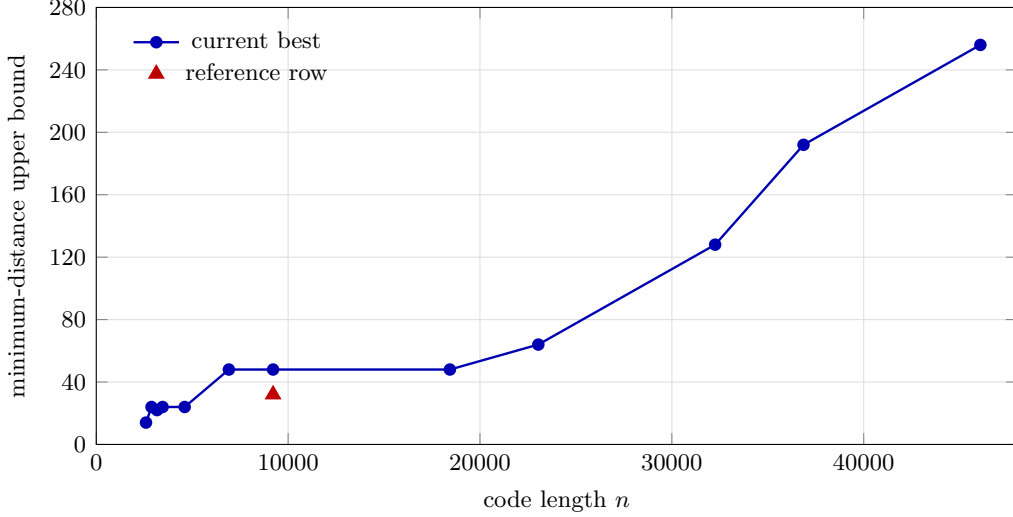
Figure 2: Current best upper bounds as a function of the code length n . The blue polyline traces the best available row found in the present search for each P , including the daggered high- P candidates when they improve the record, while the red triangle marks the non-winner reference row listed in Table 2.
