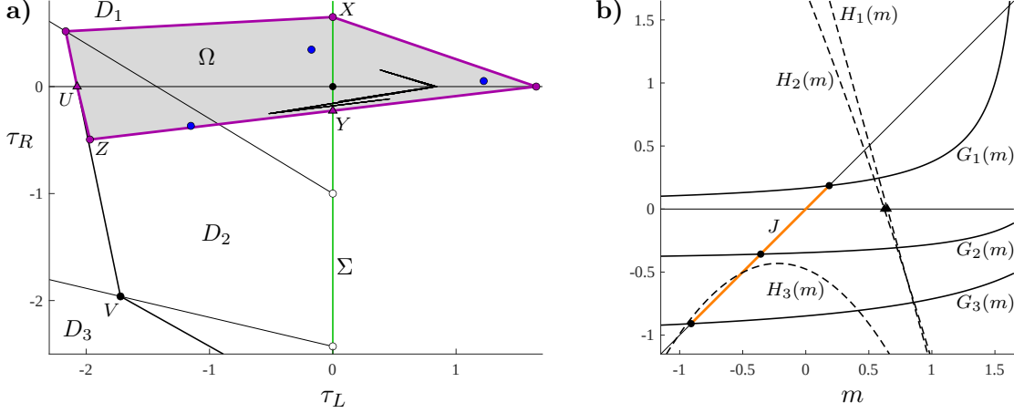
Figure 16: Constructive elements produced by Algorithm 7.1 for (2.1) with (2.2) and (\tau_L, \tau_R) = (0.7, 1.8) . Here the algorithm obtains \beta = 0.65 and returns \chi_{\text{chaos}} = \text{false} . Panel (a) shows the forward invariant region \Omega , the regions D_p , a numerically computed attractor, and a stable period-3 solution (blue circles). Panel (b) shows G_j and H_j for j = 1, 2, 3 .
